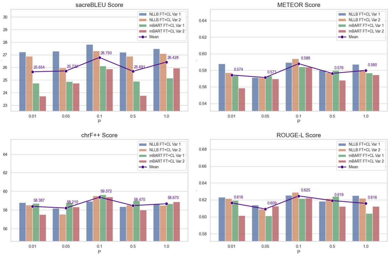
FIGURE 9. sacreBLEU, chrF++, METEOR, and ROUGE-L evaluation based on penalty value.
