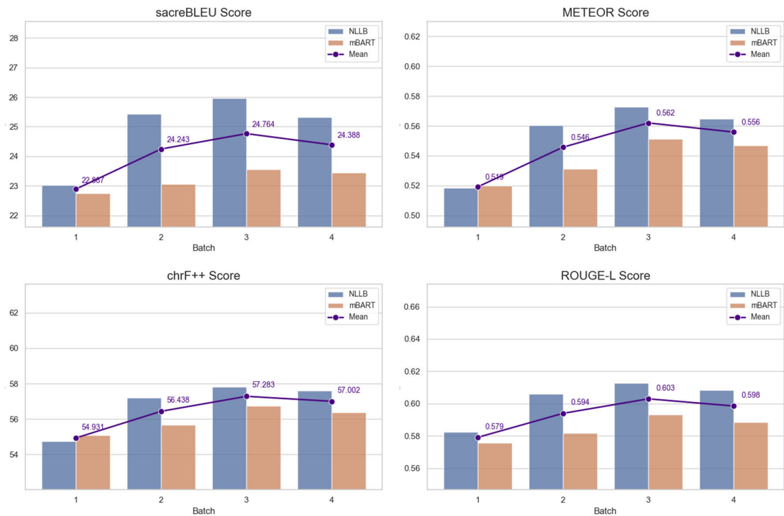
FIGURE 5. sacreBLEU, chrF++, METEOR, and ROUGE-L evaluation based on batch size.
