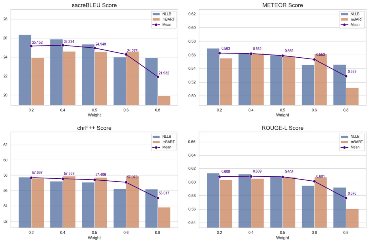
FIGURE 8. sacreBLEU, chrF++, METEOR, and ROUGE-L evaluation based on loss integration type 2 weight value.
