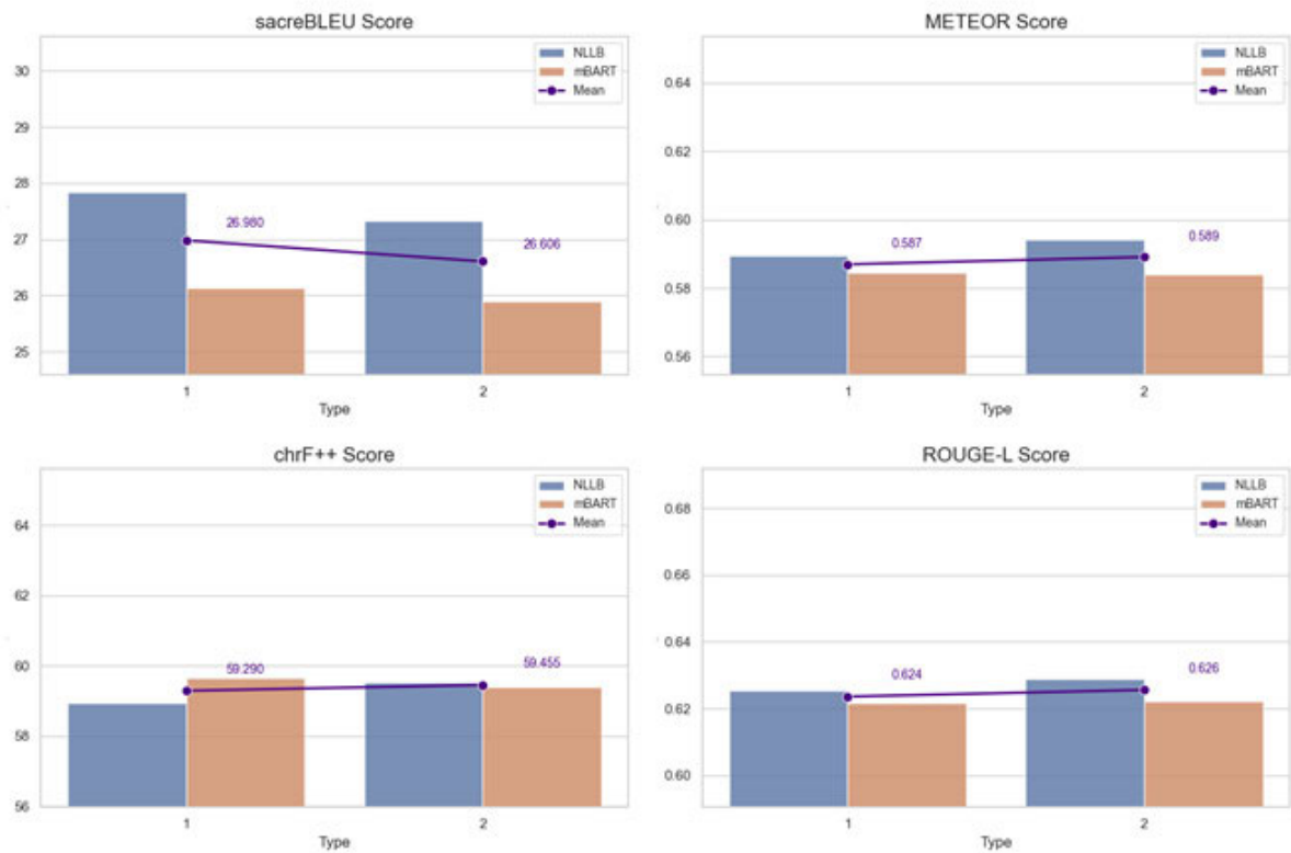
FIGURE 6. sacreBLEU, chrF++, METEOR, and ROUGE-L evaluation based on loss integration variant: custom loss directly added to total loss (integration type 1), and proportional combination of custom and standard loss (integration type 2).
