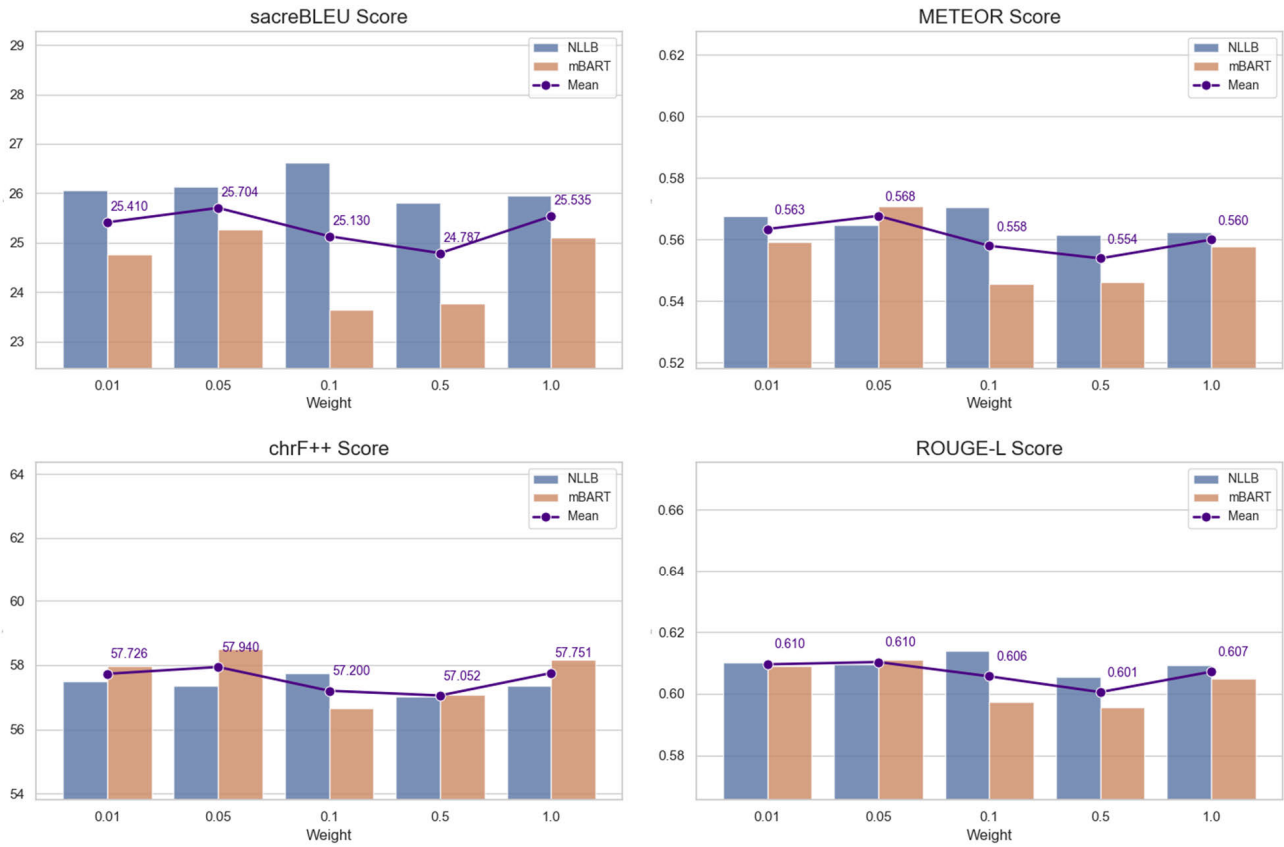
FIGURE 7. sacreBLEU, chrF++, METEOR, and ROUGE-L evaluation based on loss integration type 1 weight value.
